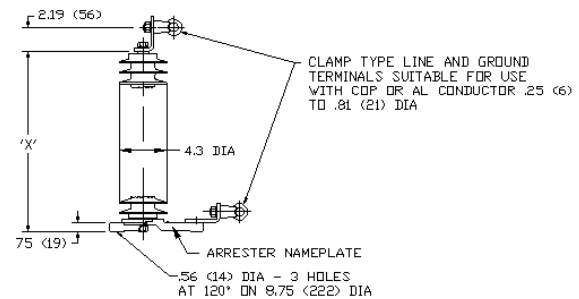
Figure 11. Polymer Intermediate Arrester, 3kV through 72kV [9L12PPBXXS]
